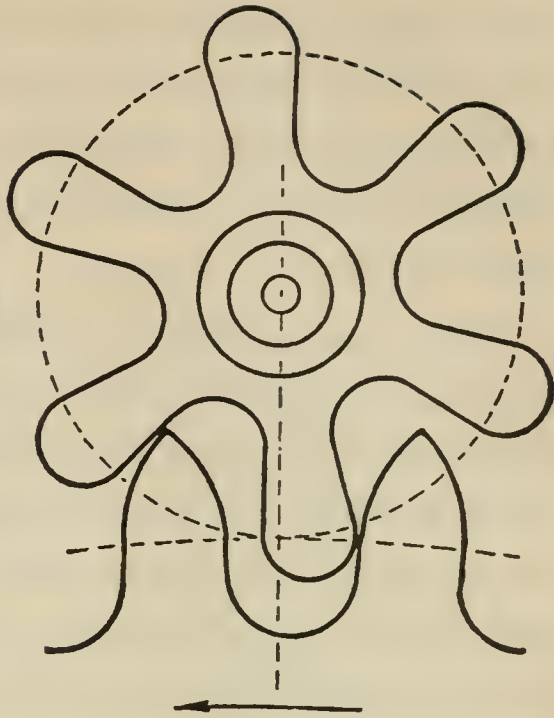
Figure 3. Six-leaf pinion.
