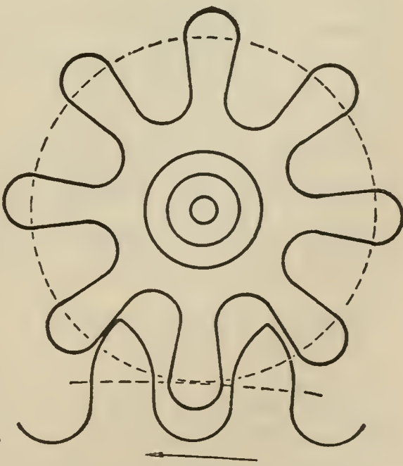
Figure 5. Pinion too small.
