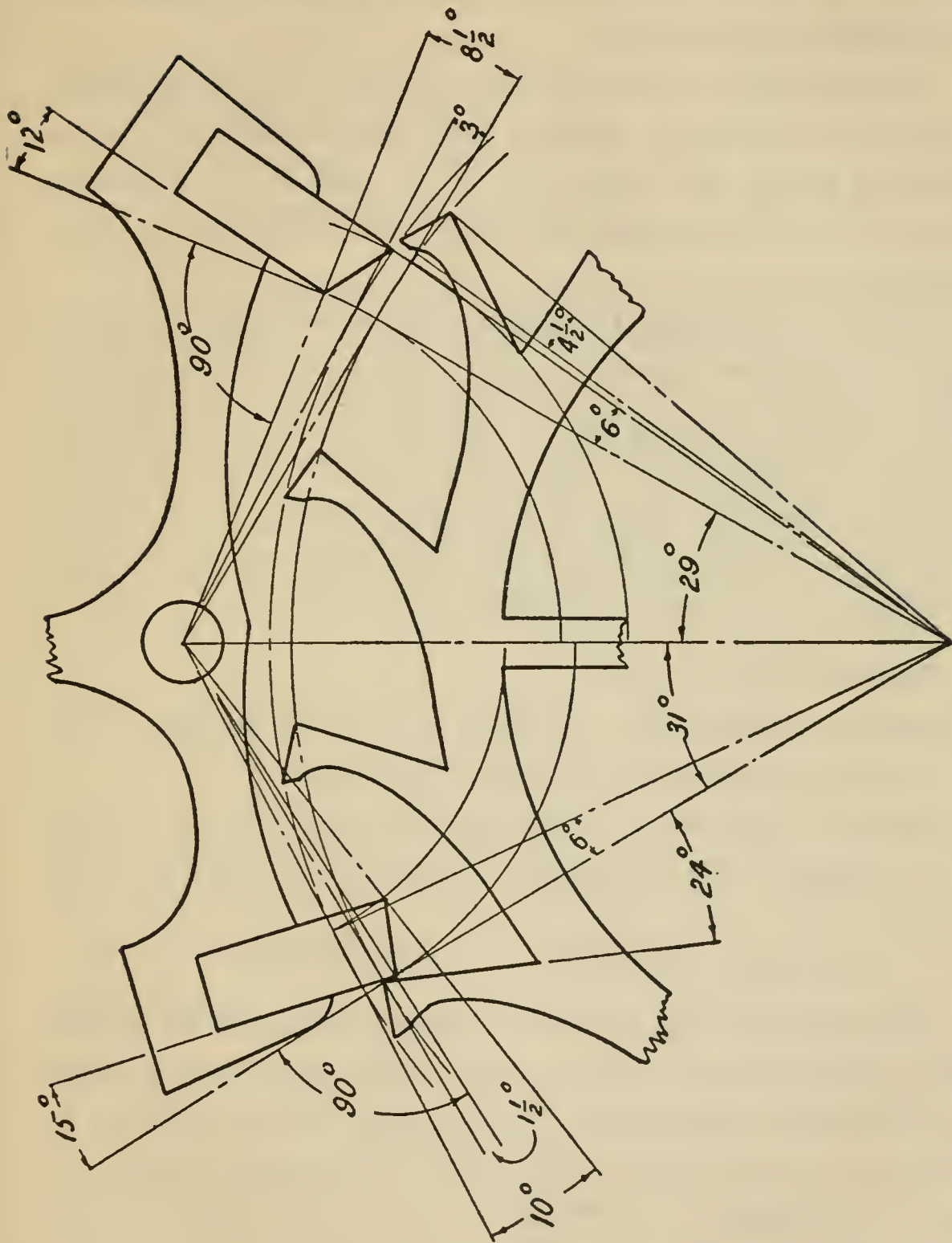
Figure 40. Semitangential escapement.
